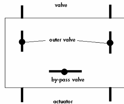
Fig. 2 • Three valve isolating manifold
